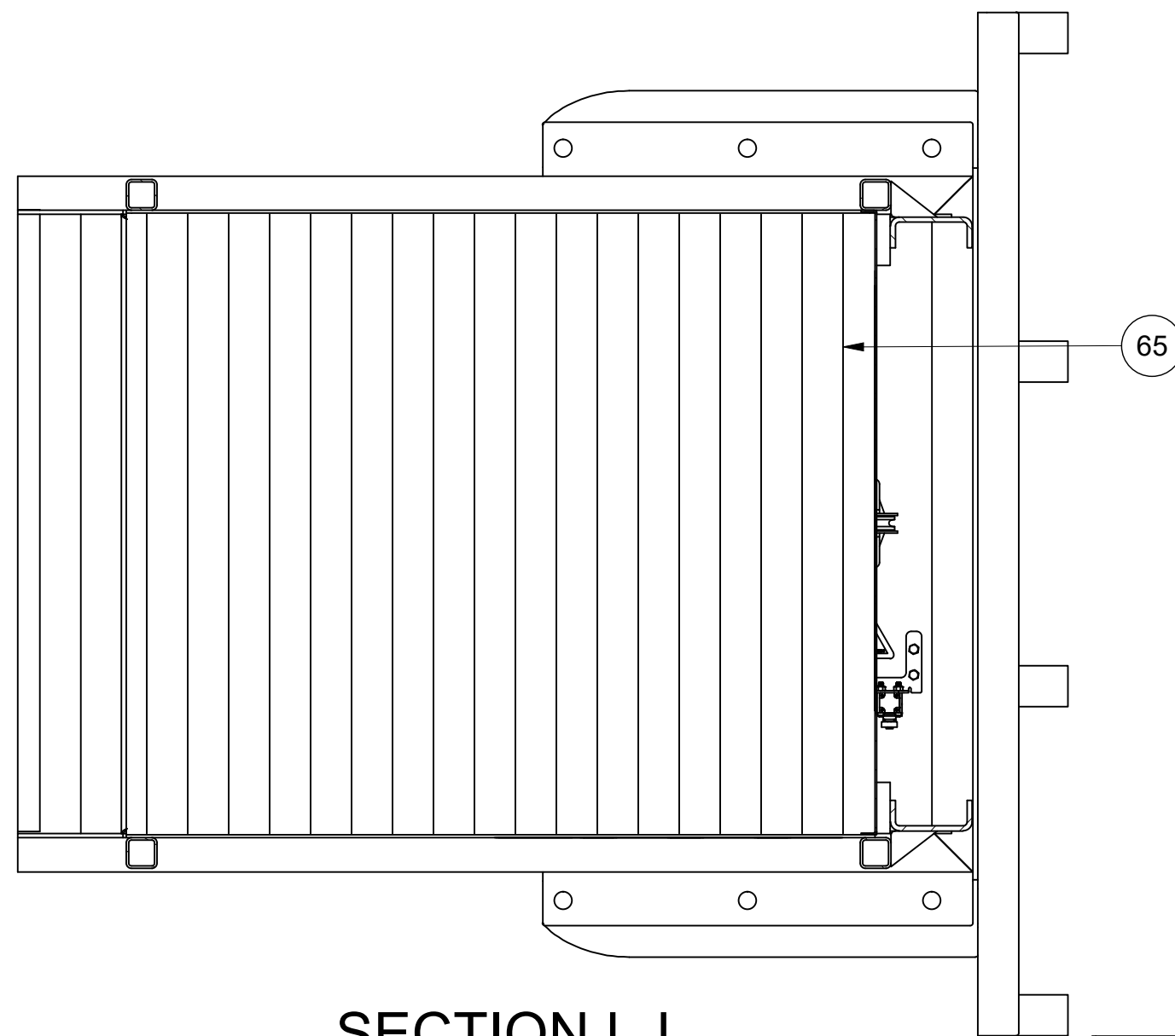
SECTION L-L SCALE 1/8" = 1"
