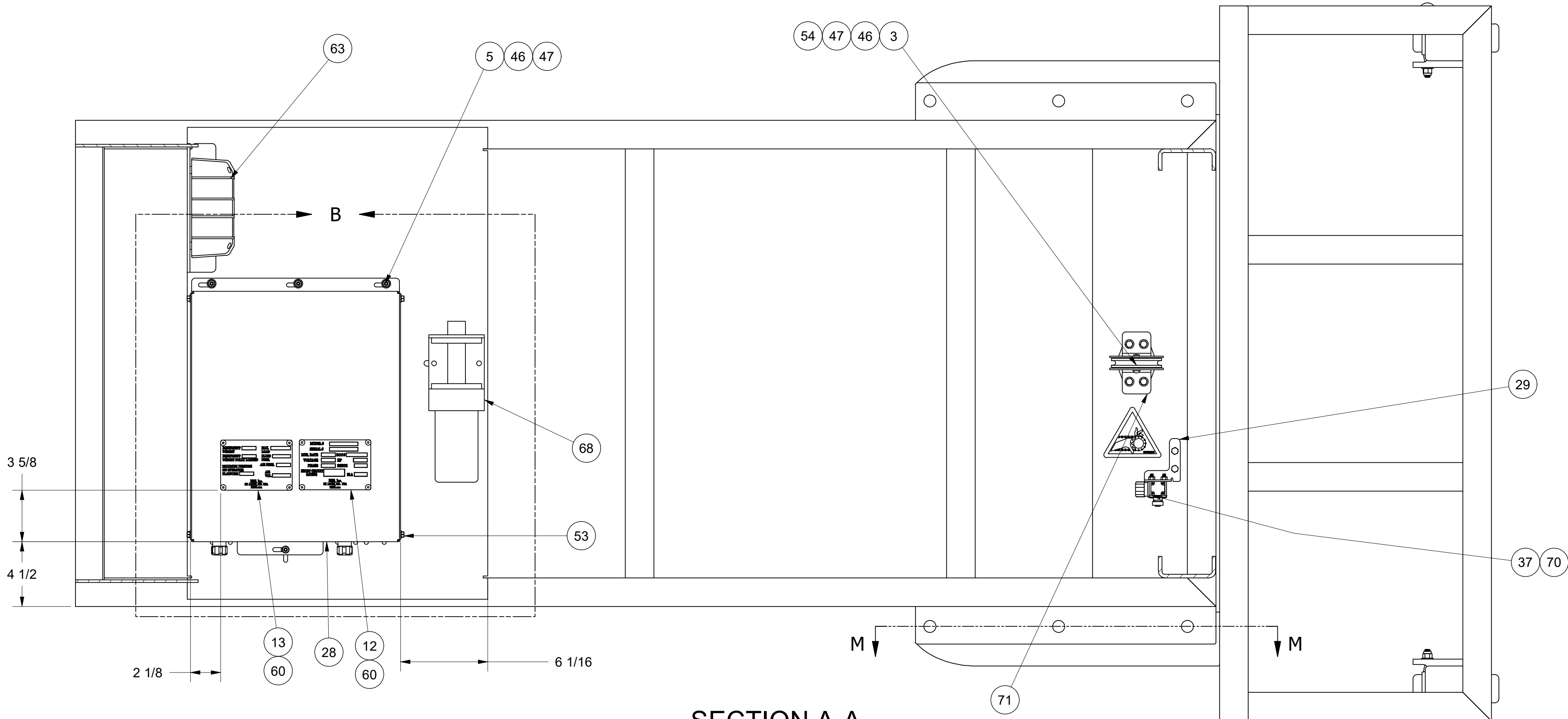
SECTION A-A SCALE 3/16" = 1"
