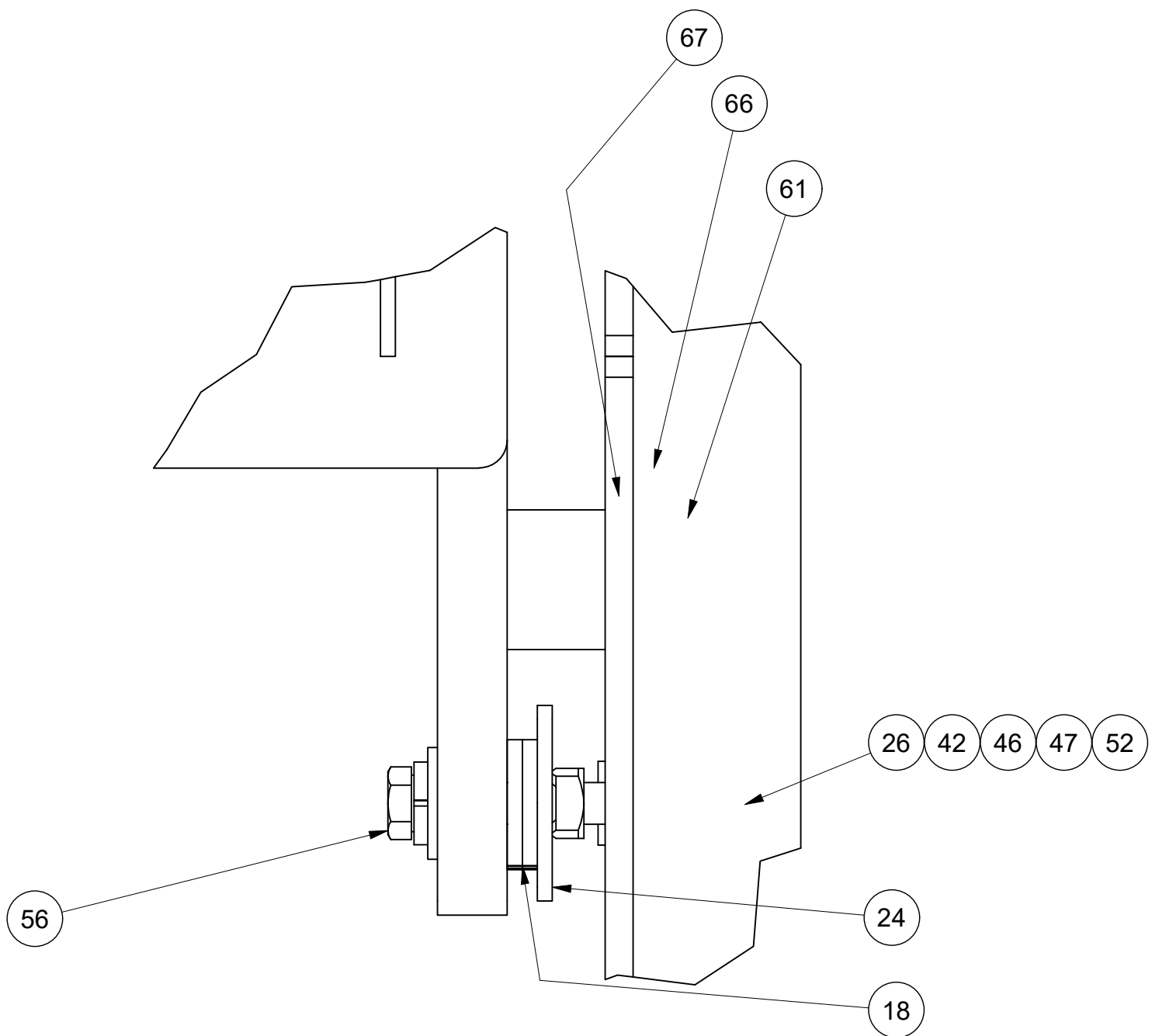
4X DETAIL E SCALE 3/4" = 1"
